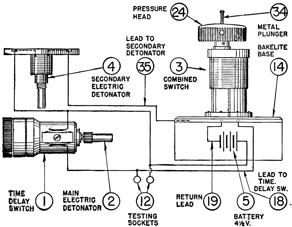
FIGURE 36.—Railway time-delay (electrically operated) mine.
